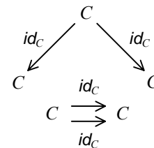
Figure 4: Unit Graph
