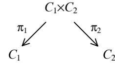
Figure 2: Binary Product
