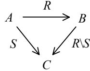
Figure 2: Left Residuation
