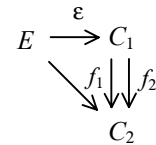
Figure 4: Equalizer
