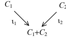
Figure 2: Binary Coproduct
