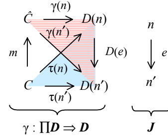
Diagram 3: Limiting Cone
