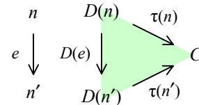
Diagram 2: Cocone
