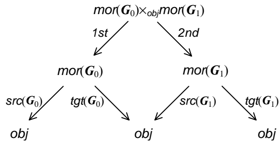
Figure 3: Multiplication Graph
