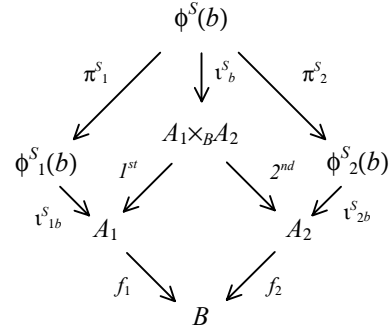
Figure 7: Pullback Fibers
