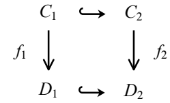
Diagram 1: Restriction
