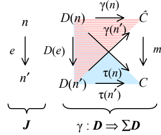
Diagram 3: Colimiting Cocone
