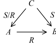
Figure 3: Right Residuation
