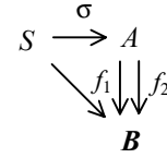
Figure 8: Subequalizer
