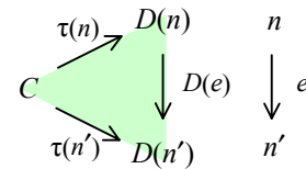
Diagram 2: Cone
