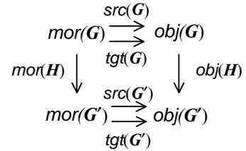
Figure 5: Graph Morphism
