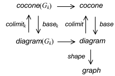
Diagram 1: Diagrams, Cocones and Fibers
