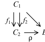
Figure 4: Coequalizer
