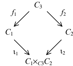
Figure 5: Pushout
