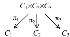
Figure 3: Ternary Product
