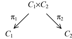
Figure 2: Binary Product
