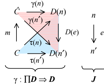
Diagram 3: Limiting Cone
