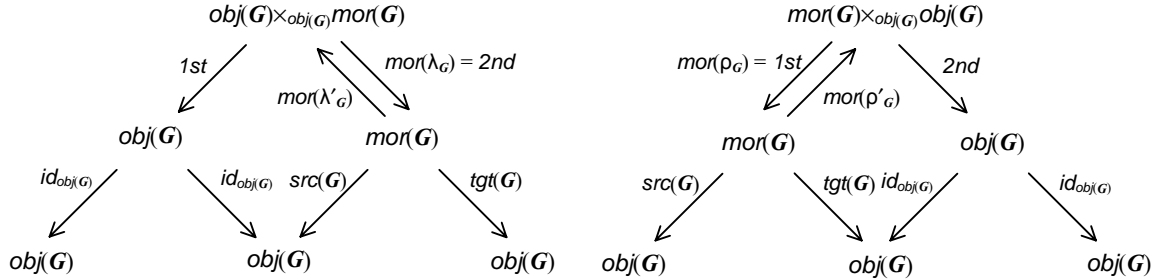
Figure 8: Left Unit and Right Unit Graph Isomorphism
