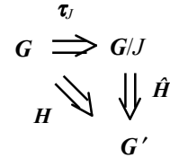
Figure 8: Universality of the quotient
