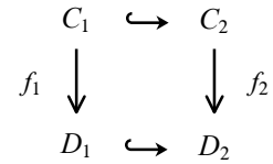
Diagram 1: Restriction
