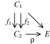
Figure 4: Coequalizer
